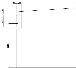
PARTITION WALL DETAIL VIEW X-X
